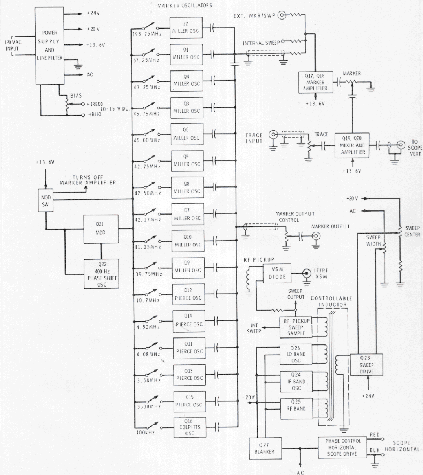
BLOCK DIAGRAM
