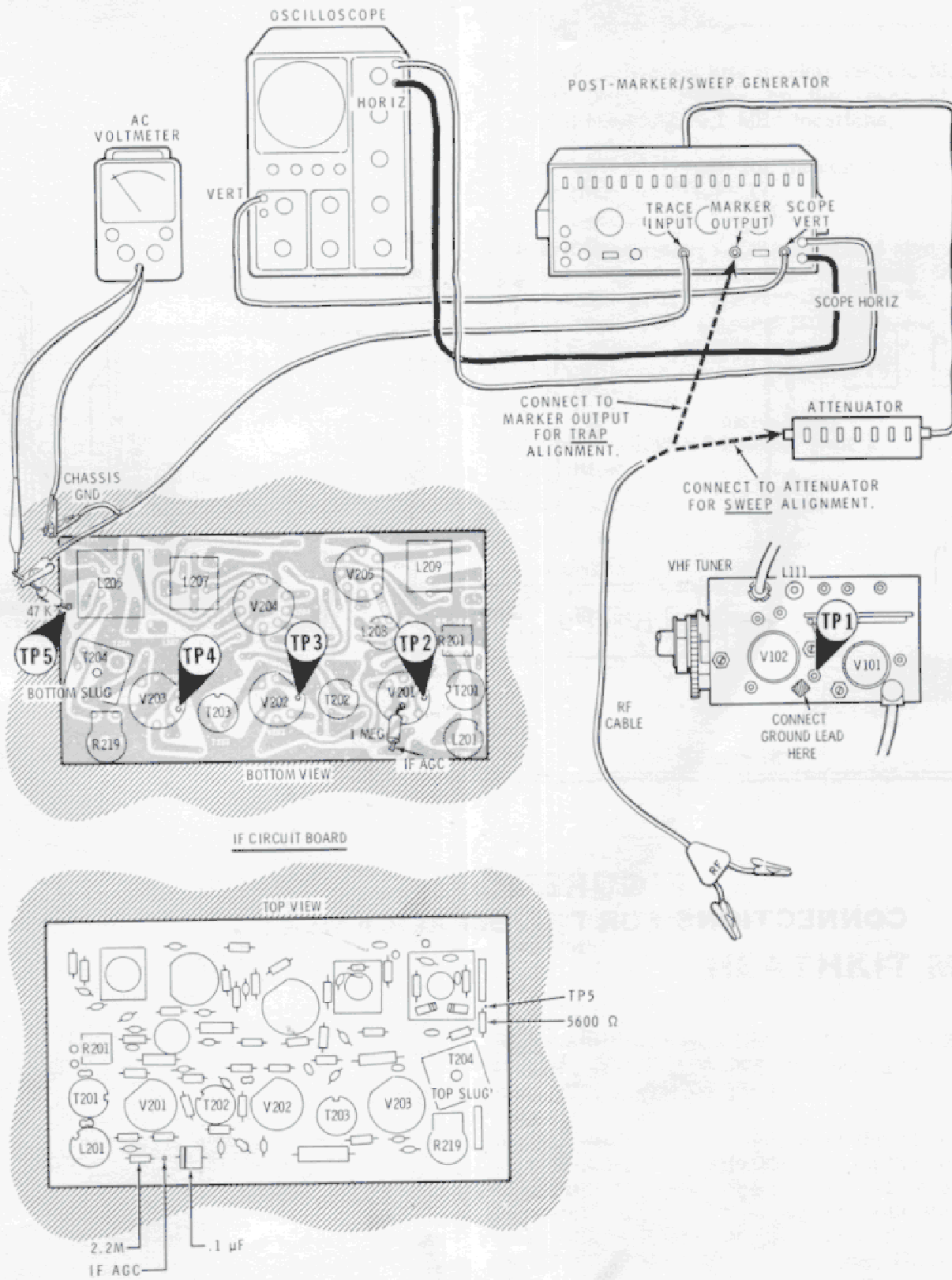
FIGURE 19 SWEEP ALIGNMENT
